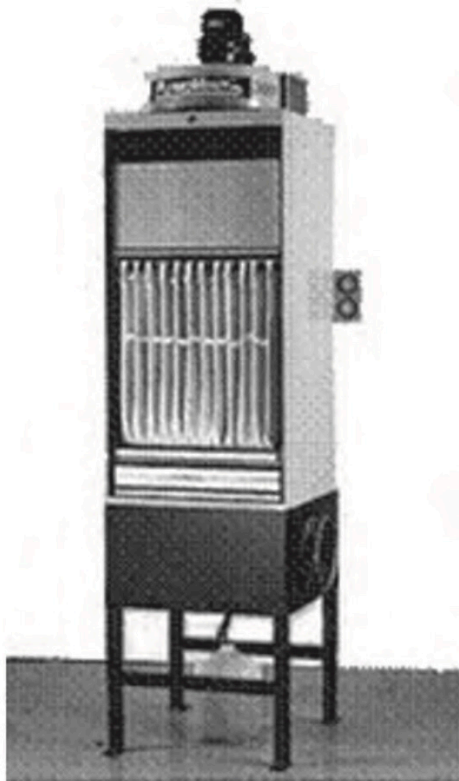
Figure 5: Progressive filtration unit with spark arrestor, MERV 14 filter and HEPA final filter configuration. Courtesy Plymovent North America
